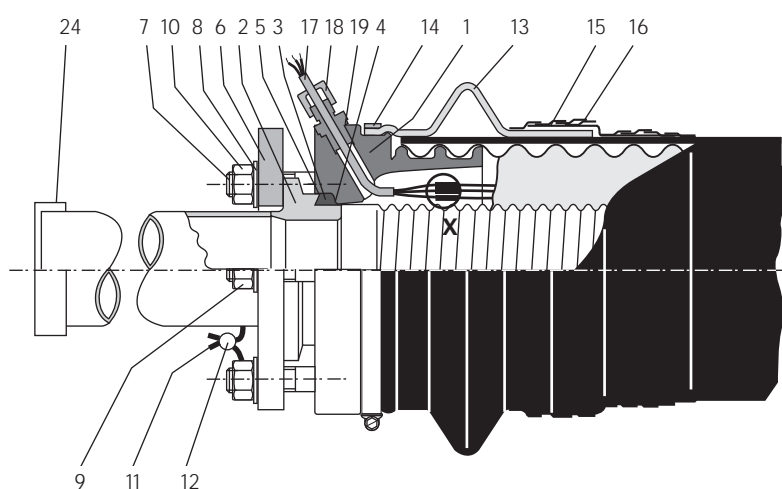
Figure 1: Raccord (type A)
