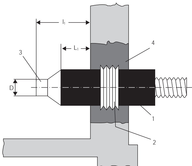
Figure 1: Raccord de type G, soudé
